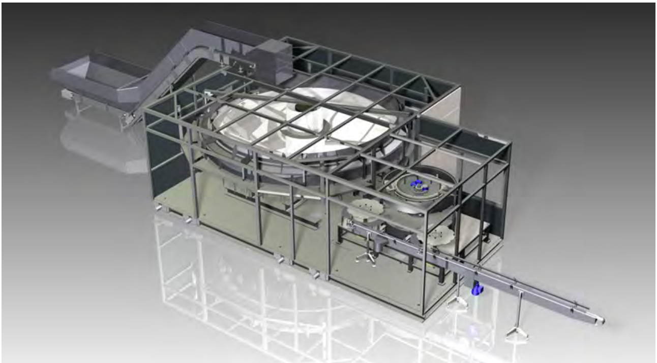
Interior part of unscrambler MONOCHUTE-50 with integrated Rotary Orientor in monoblock. (Simulation 3D).
